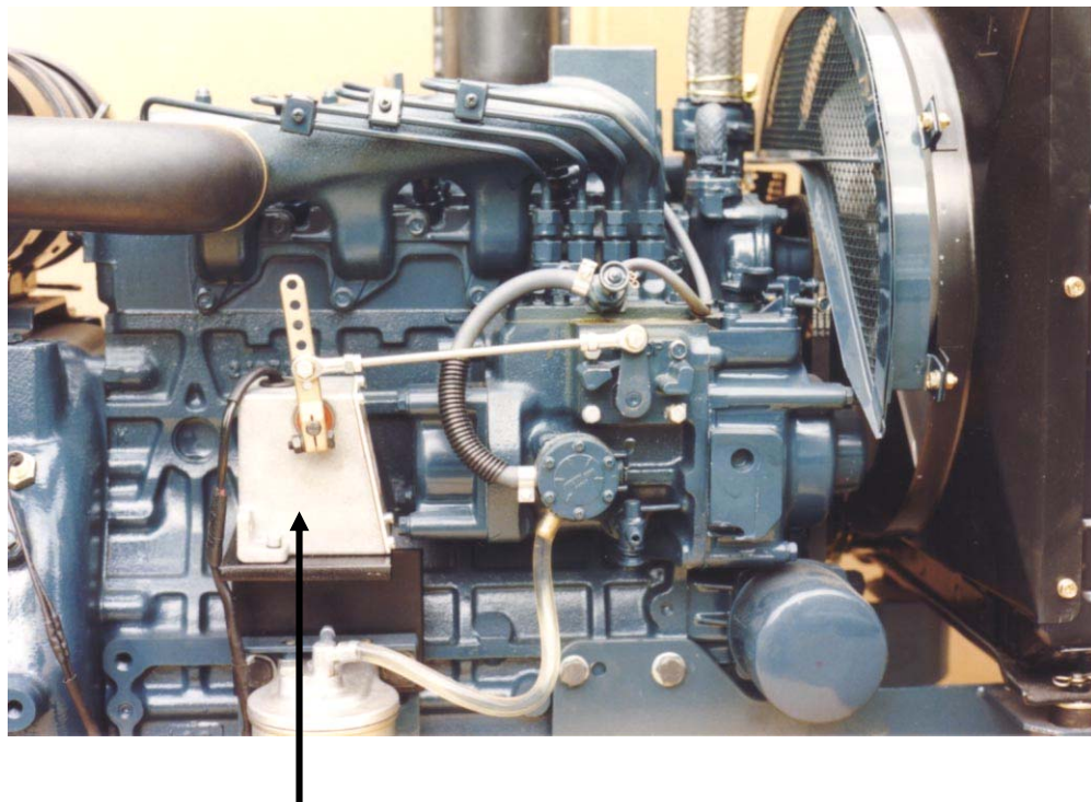
ADD 120S-12 Actuator
