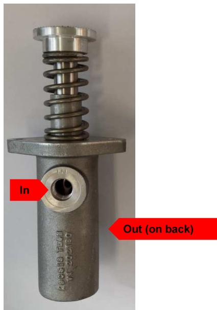
Fig. 1: Adapter SAE 6 to 3/8" NPTF for In-/Outlet ports.
