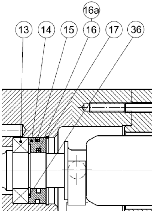
Service Kit KT-3-361 to HCD Drive shaft
