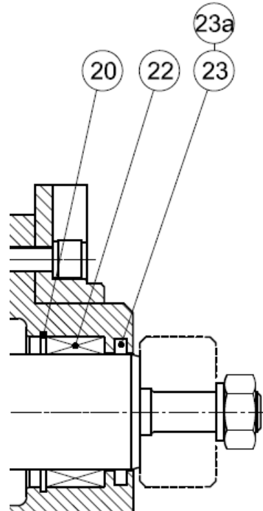
Service Kit KT-3-353 to HCD Drive housing
